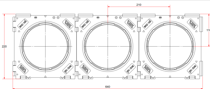
BKD150-K2 without spacer (ASH)
