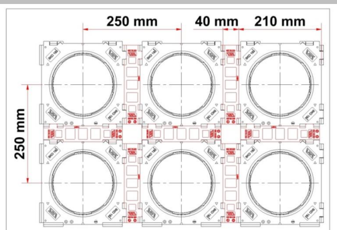
BKD150-K2 with spacer (ASH)
