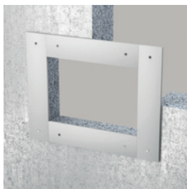
Fig. 2: Board frame for rigid floor and flexible wall (arranged either on one side or both sides, thickness of the board frame per side, max. 50 mm)
